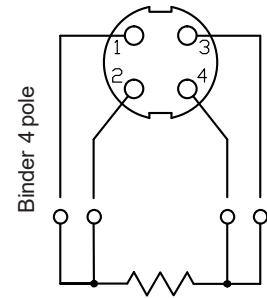
Connector pin-out
